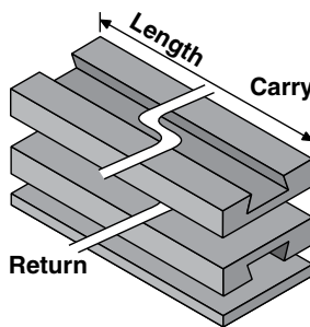
Straight Track
