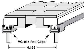
Tab Chain Guide mounting options
