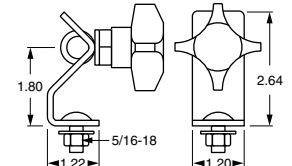
VG-223RN-TOP
