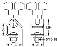
VG-213RN-TOP
