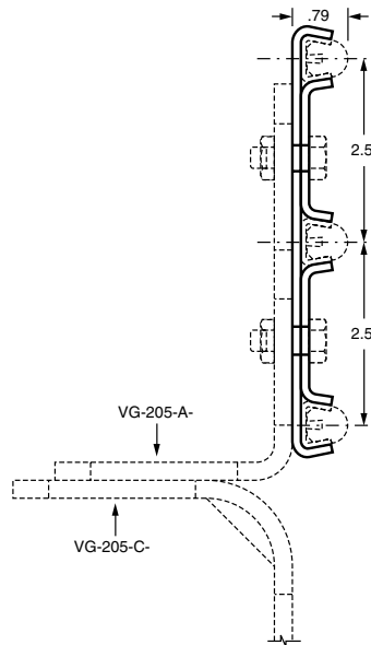
VG-011-02-SH
