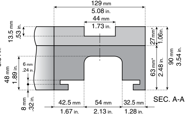
ONE TRACK
